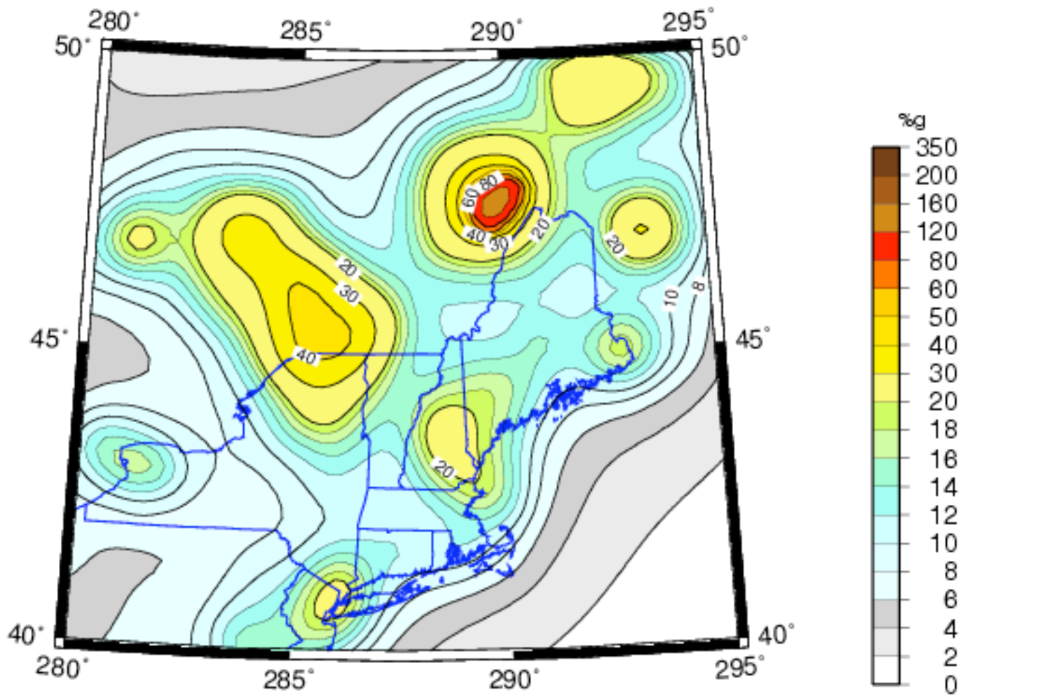
Peak Acceleration (%g) with 2% Probability of Exceedance in 50 Years site: NEHRP B-C boundary U.S. Geological Survey National Seismic Hazard Mapping Project
