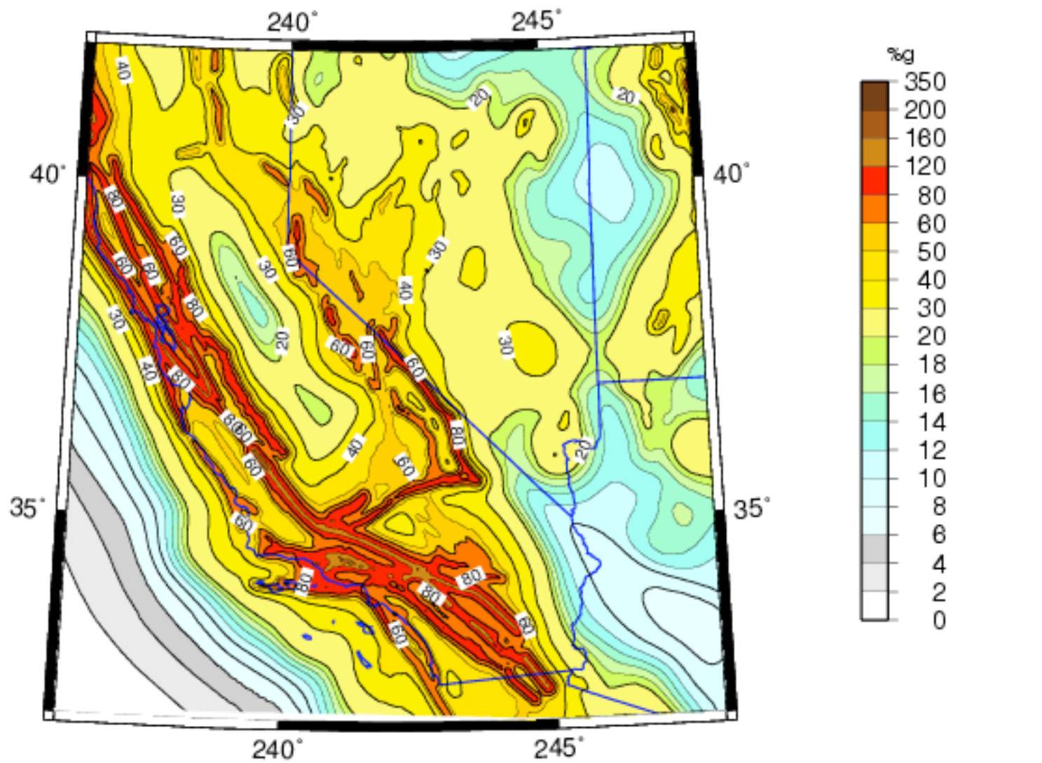
Peak Acceleration (%g) with 2% Probability of Exceedance in 50 Years site: NEHRP B-C boundary U.S. Geological Survey National Seismic Hazard Mapping Project
